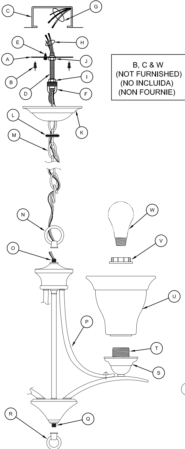
DIAGRAM - A 4326
